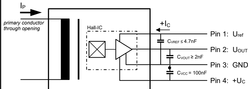
Fig. 6: functional block diagram of the sensor
